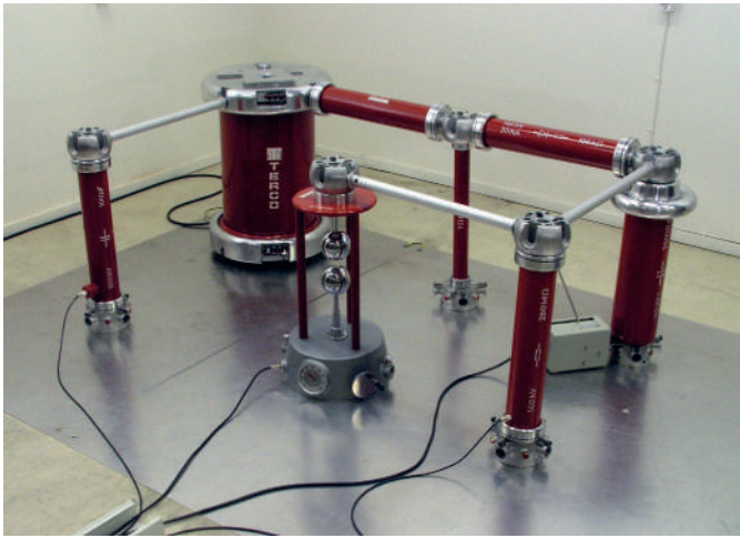
Measurement of flashover
