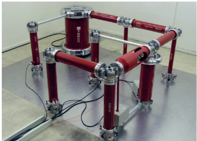
Impulse Set-up
