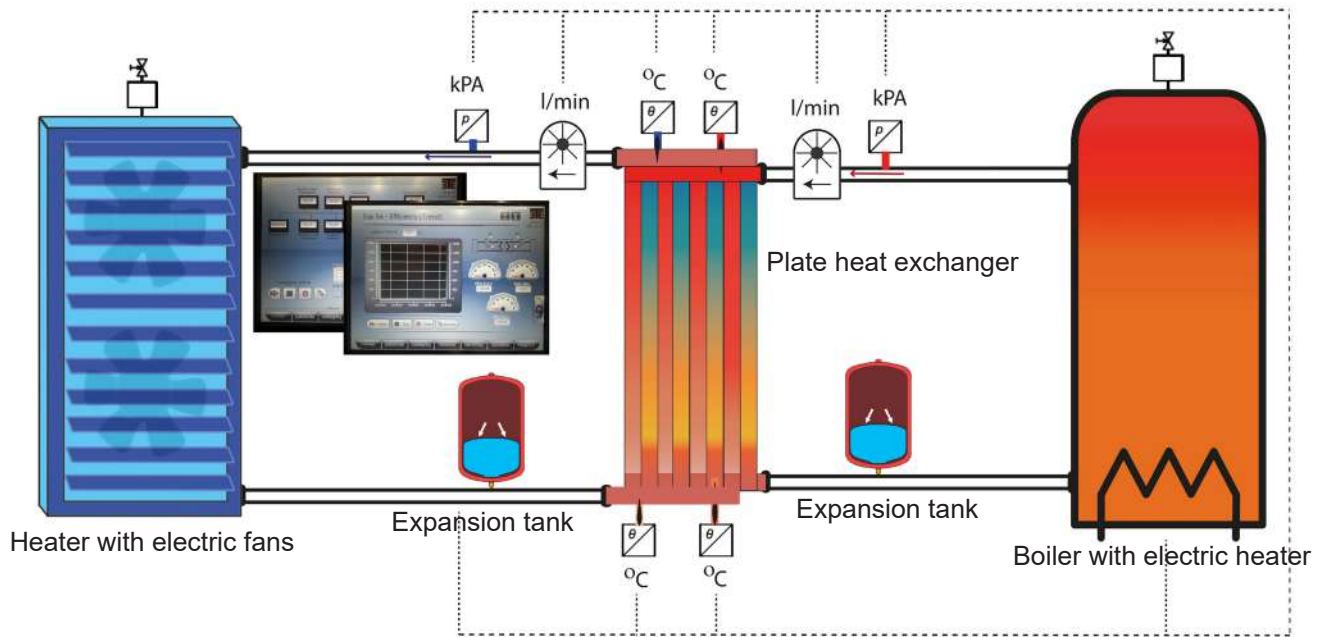
Principle Diagram
