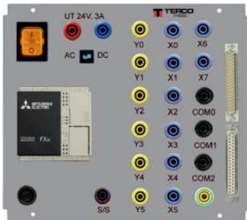
TF8050-FX3s PLC-module Mitsubishi Melsec-FX3s 6 input, 8 output Current max for application:24V, 3A
