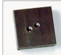
Brinell Test Piece after Brinell Indent
