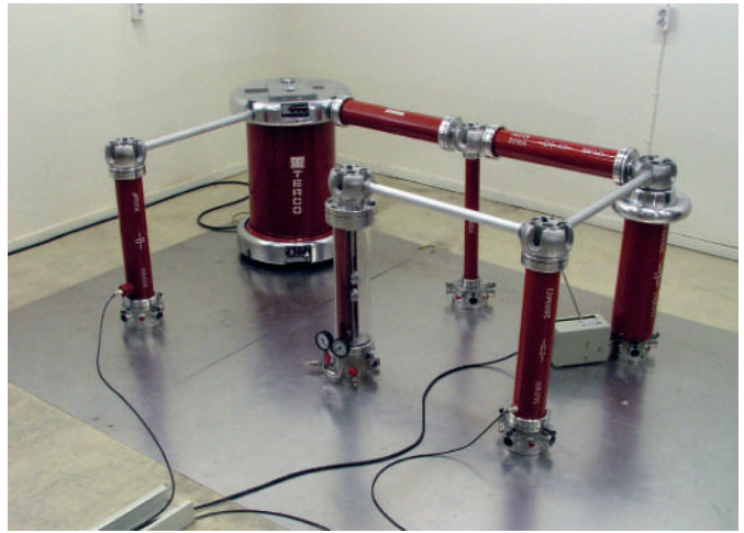
Measurement of flashover voltage in vacuum and under pressure
